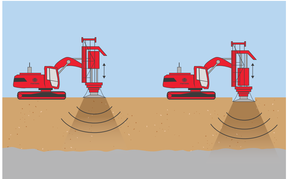
Rapid Impact Compaction (RIC) is performed by repeatedly driving a steel plate into the ground in a predetermined grid pattern.
