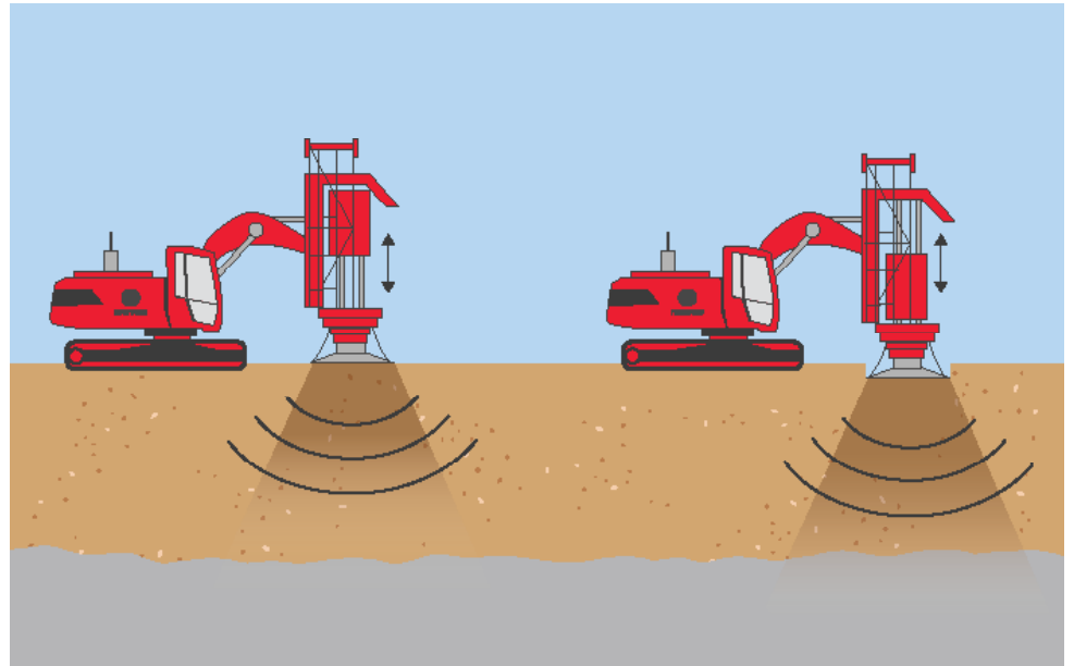
Rapid Impact Compaction (RIC) is performed by repeatedly driving a steel plate into the ground in a predetermined grid pattern.
