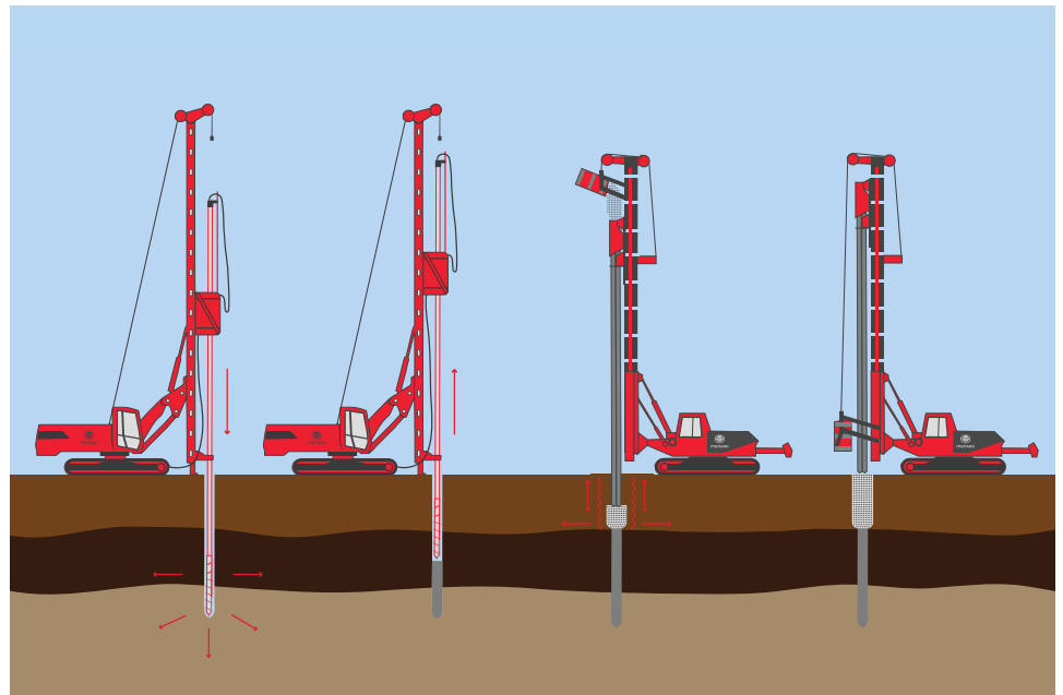
CMC installed with displacement drilling methods (left). Stone column installed on top of CMC with stone column equipment (right).
